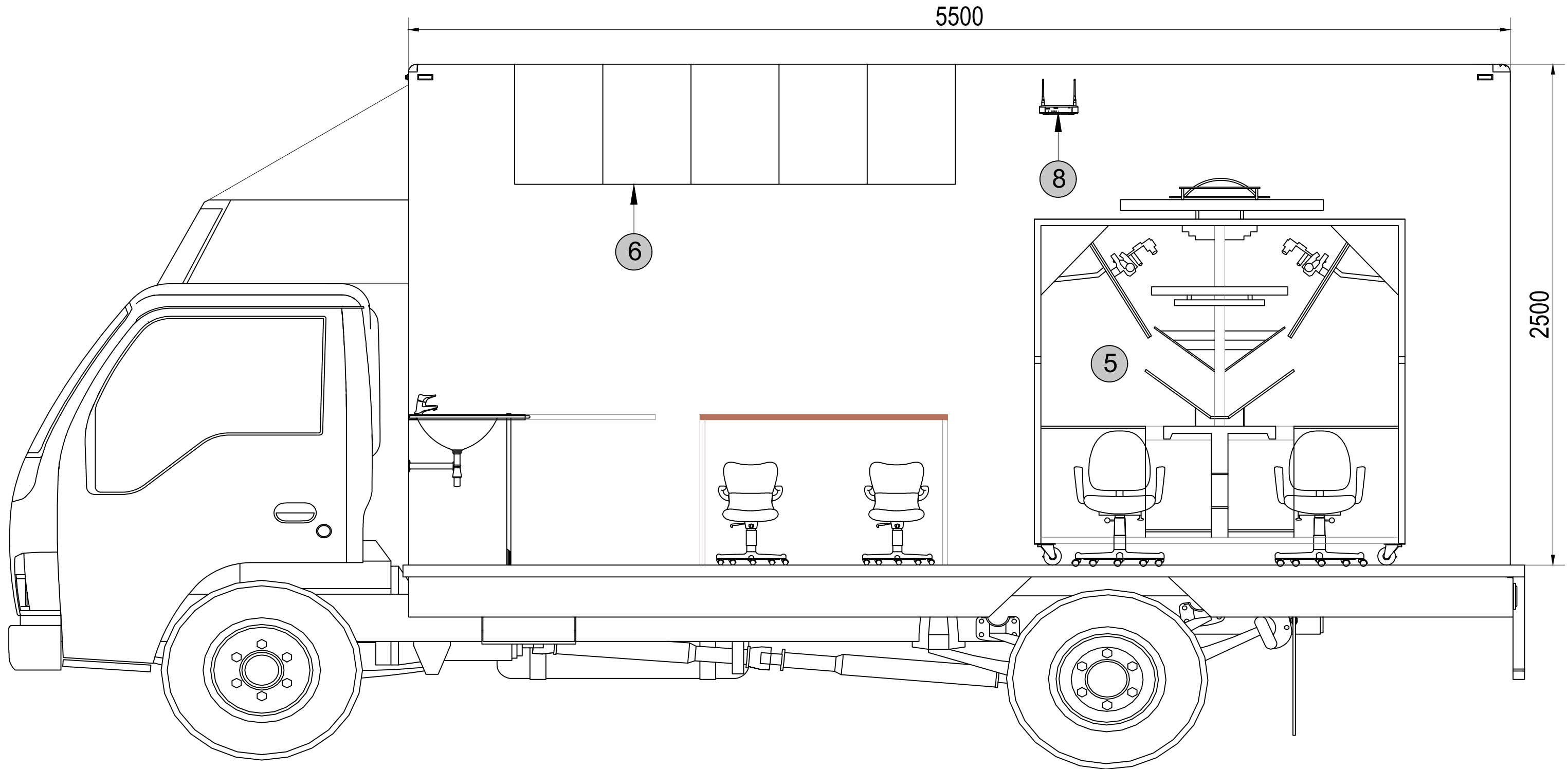
INTERIOR ELEVATION
